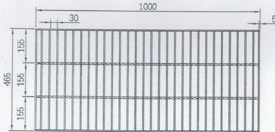
TOP VIEW SCALE 1:10
